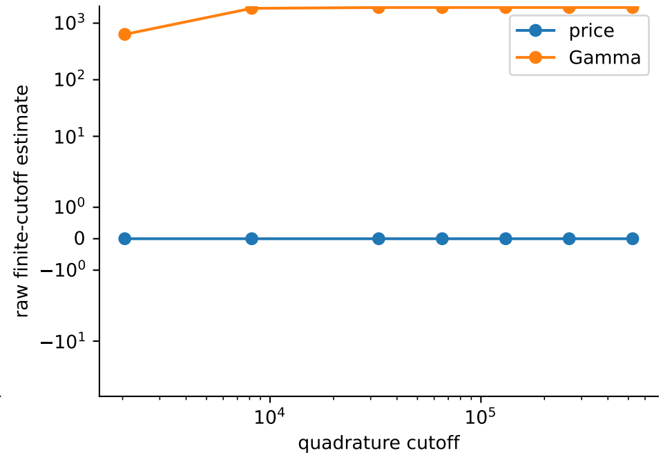
HP_ZERO_R0_EXTENDED: digit agreement does not certify the integration tail
