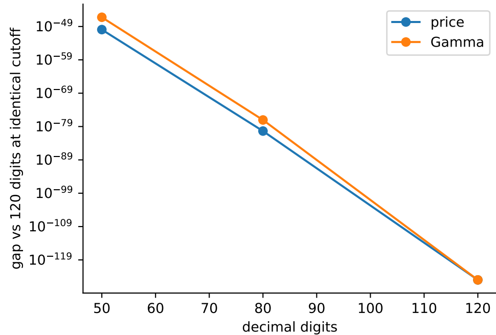
HP_ZERO_R4: digit agreement does not certify the integration tail
