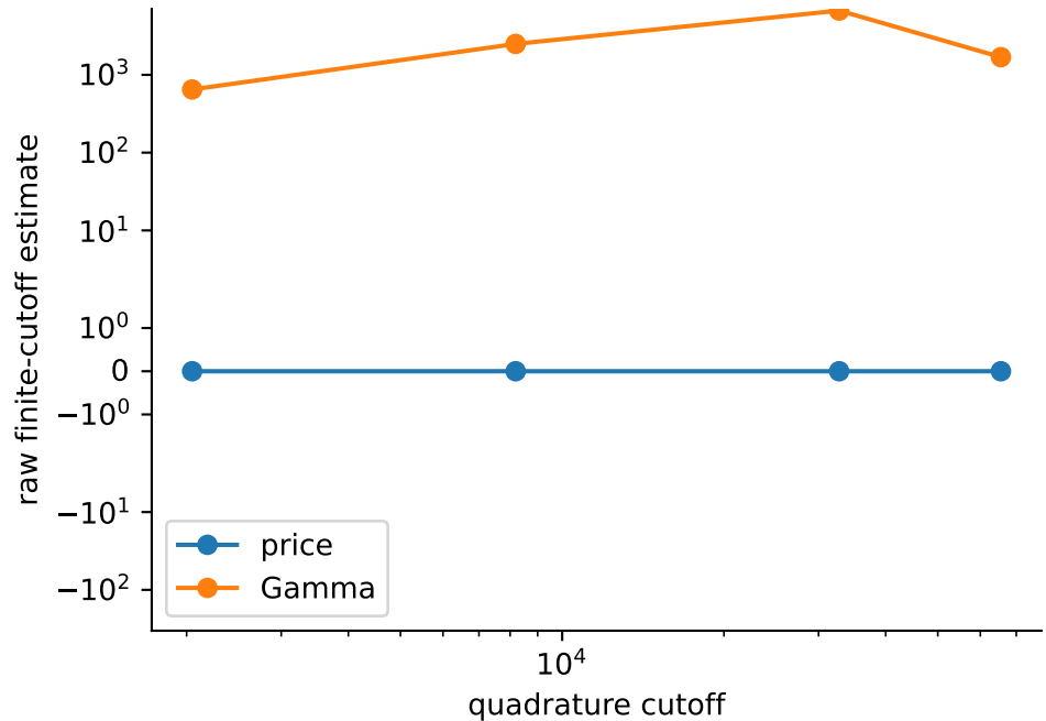
HP_ZERO_R4: digit agreement does not certify the integration tail
