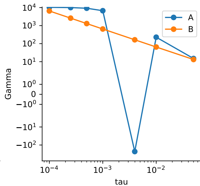
R4: maturity sequence — finite cutoffs, unresolved rows retained
