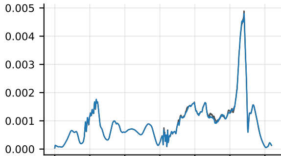
Total time
