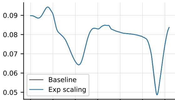
ADMM iterations
