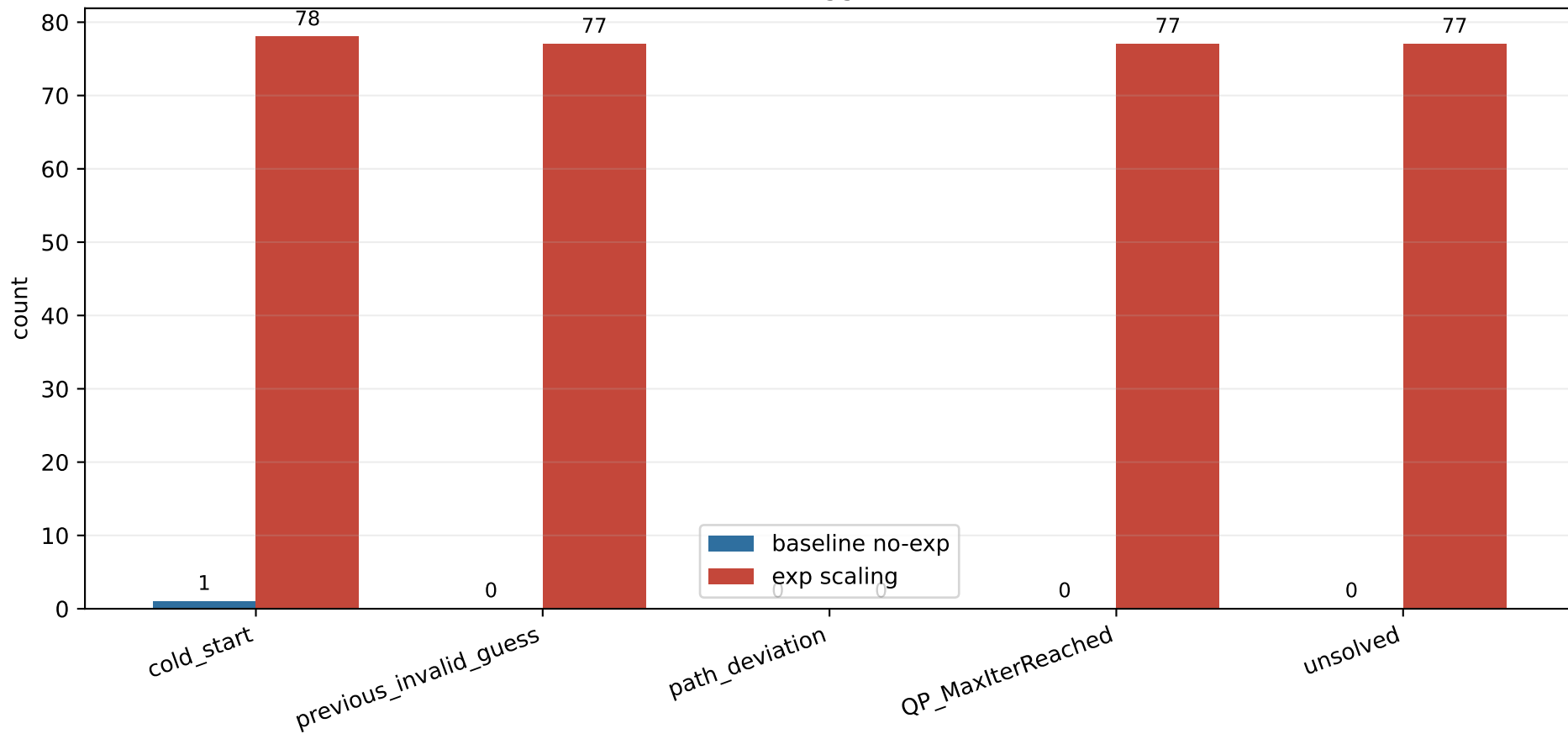
Fallback trigger counts
