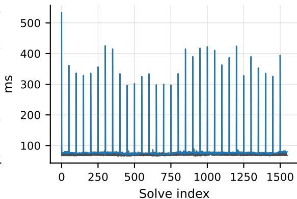
Total time
