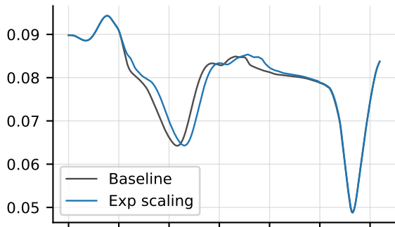
ADMM iterations
