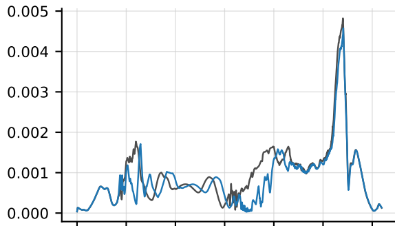
Total time
