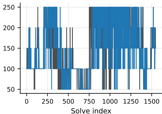
ADMM iterations
