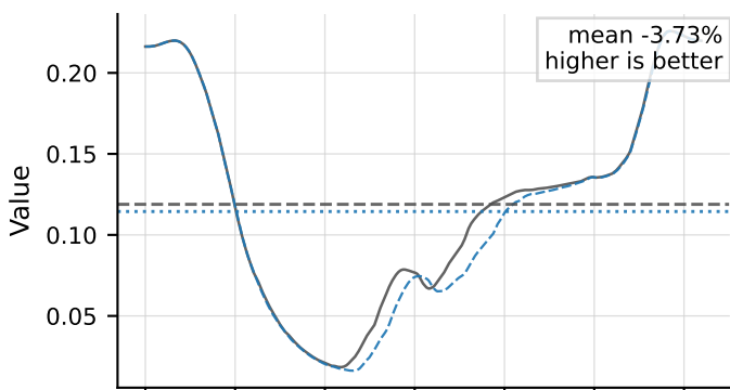
ADMM iterations
