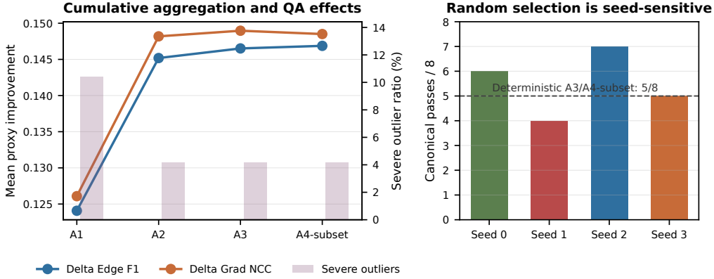
Figure 5: Cumulative ablation and random-selection supplement. Robust scene consensus improves proxy quality before the final gate, while the random-selection variant shows non-trivial seed sensitivity on the same fixed 8-scene subset.
