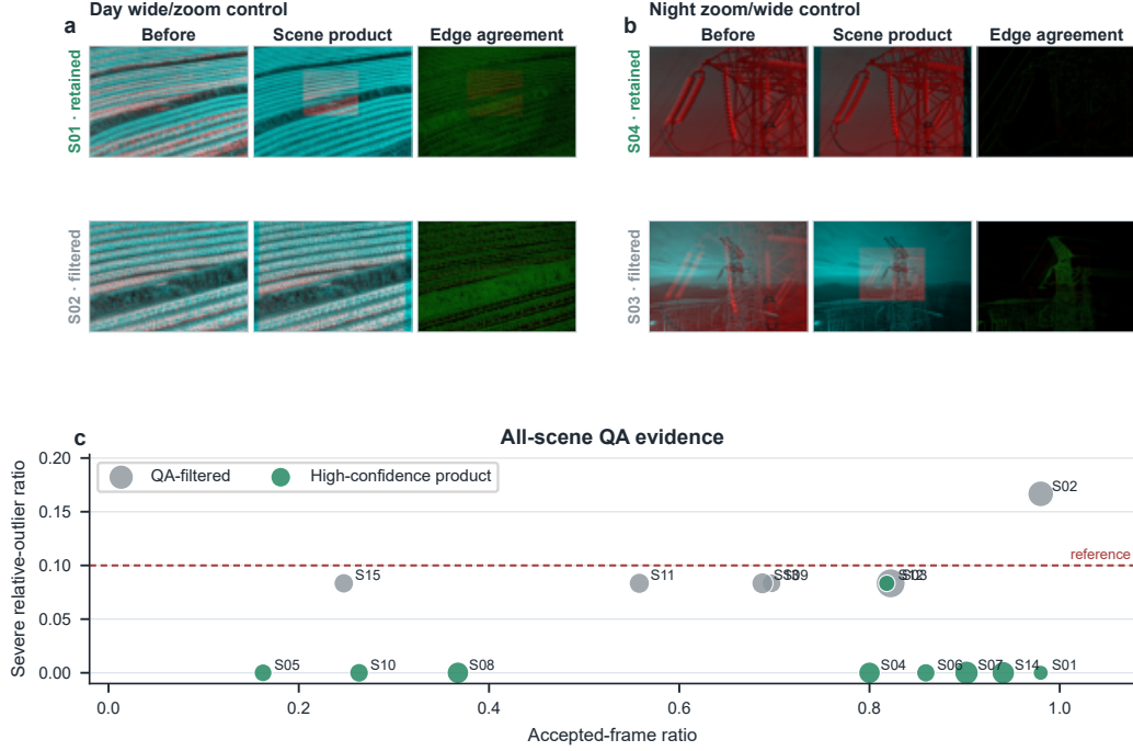
Figure 7: Reliability-controlled selection under matched scene conditions. (a,b) Wide/zoom and night paired controls show that strong pairwise support can coexist with different canonical scene outcomes. (c) Across all 15 scenes, canonical products occupy the low severe-outlier region, while accepted-frame ratio alone does not determine retention. Marker size encodes robust-rejection ratio.
