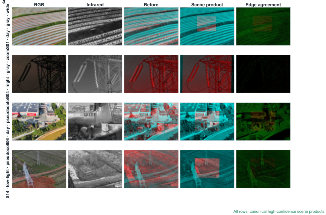
Figure 6: Representative high-confidence UAV-TAlign scene products at the canonical operating point. Rows cover day, night, and low-light scenes with grayscale and native pseudocolor infrared rendering. Columns show the RGB crop, infrared crop, unaligned overlay, scene-homography overlay, and edge-agreement visualization.
