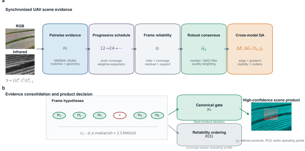
Figure 3: UAV-TAlign scene-level alignment framework. (a) Synchronized RGB-infrared pairs pass through pairwise homography generation, progressive evidence scheduling, geometry-calibrated frame reliability, robust median/MAD consensus, and cross-modal QA. (b) Unsupported frame hypotheses are rejected before the fixed canonical gate defines high-confidence products; an interpretable score independently orders operating points for coverage analysis.
