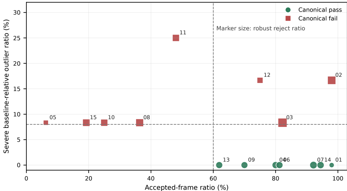
Scene-level QA separates reliable passes from fail-side outlier patterns
