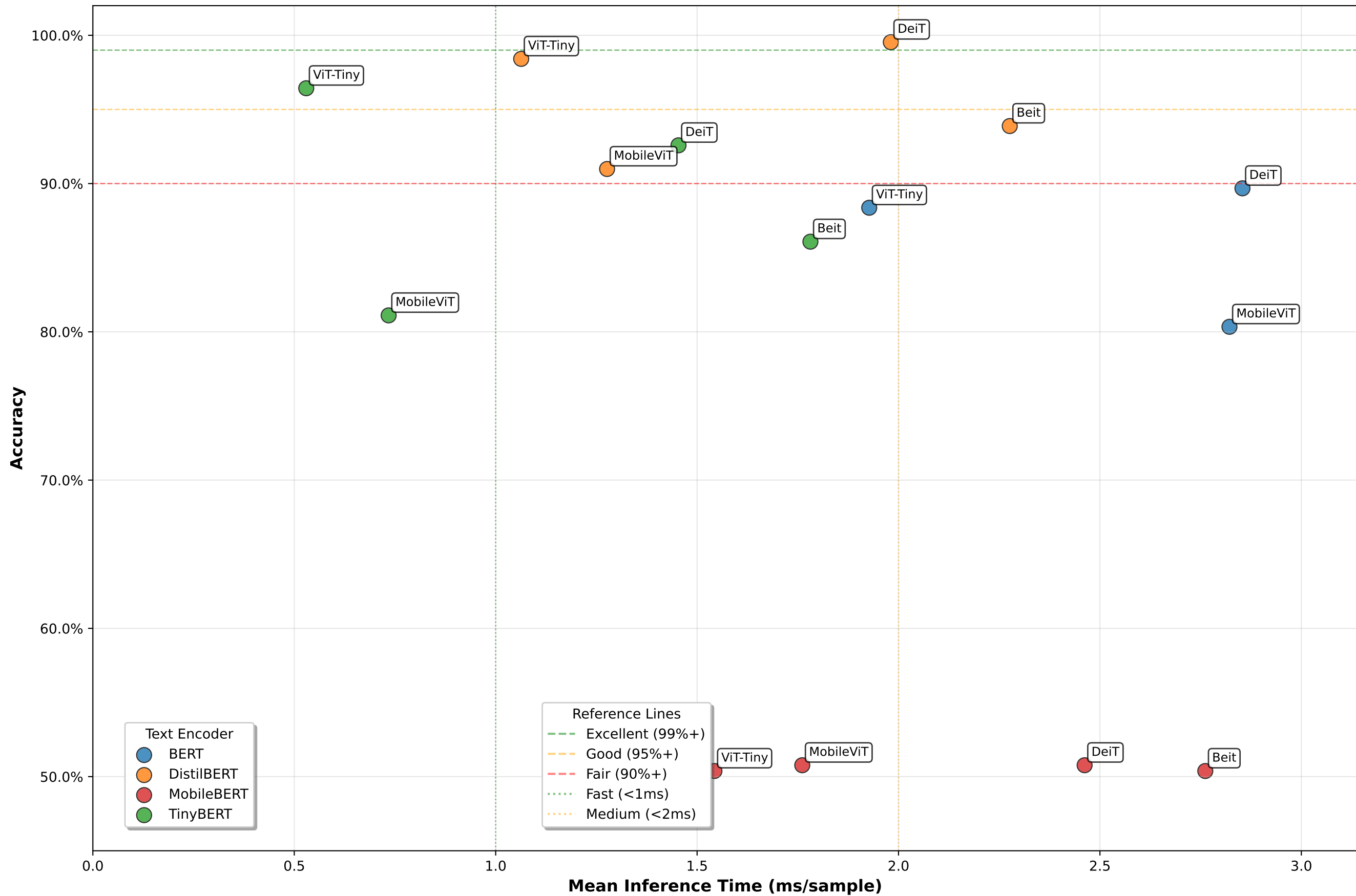
Model Inference Time vs Accuracy (Multi-Modal Text Detection Models)
