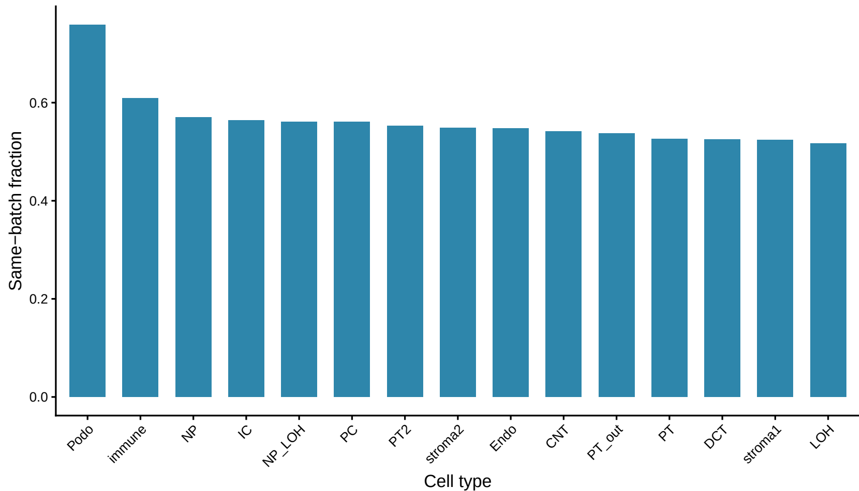
GEO precomputed UMAP P56 by-celltype same-batch fraction
