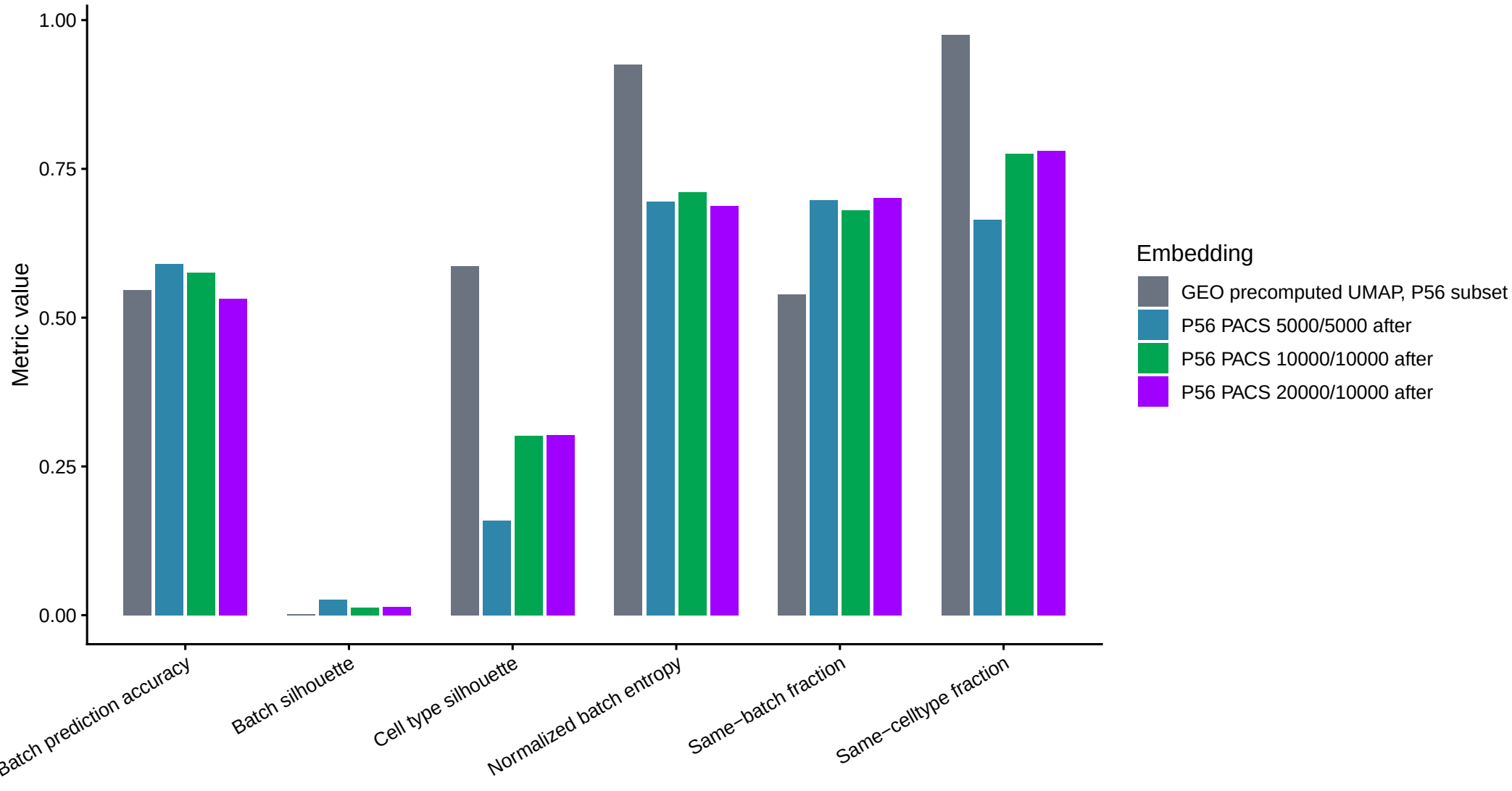
GEO precomputed UMAP vs P56 PACS-filtered UMAP metrics
