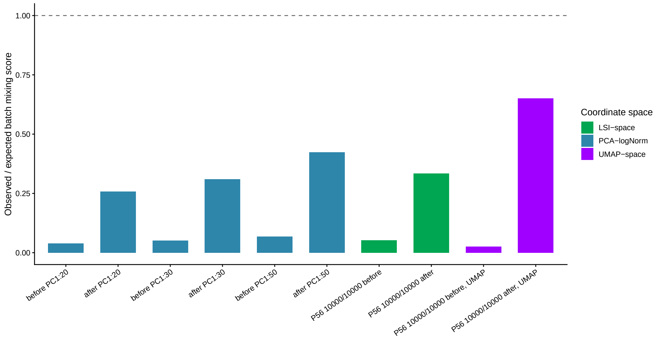
P56 10000/10000 paper-style batch mixing: PCA-logNorm vs LSI vs UMAP
