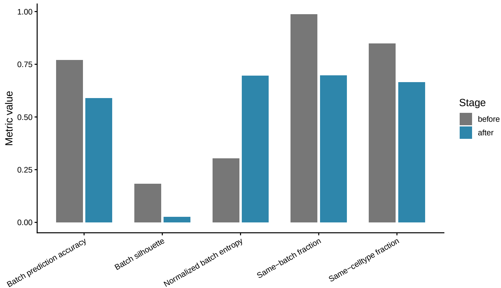
P56 before/after PACS filtering batch-mixing metrics
