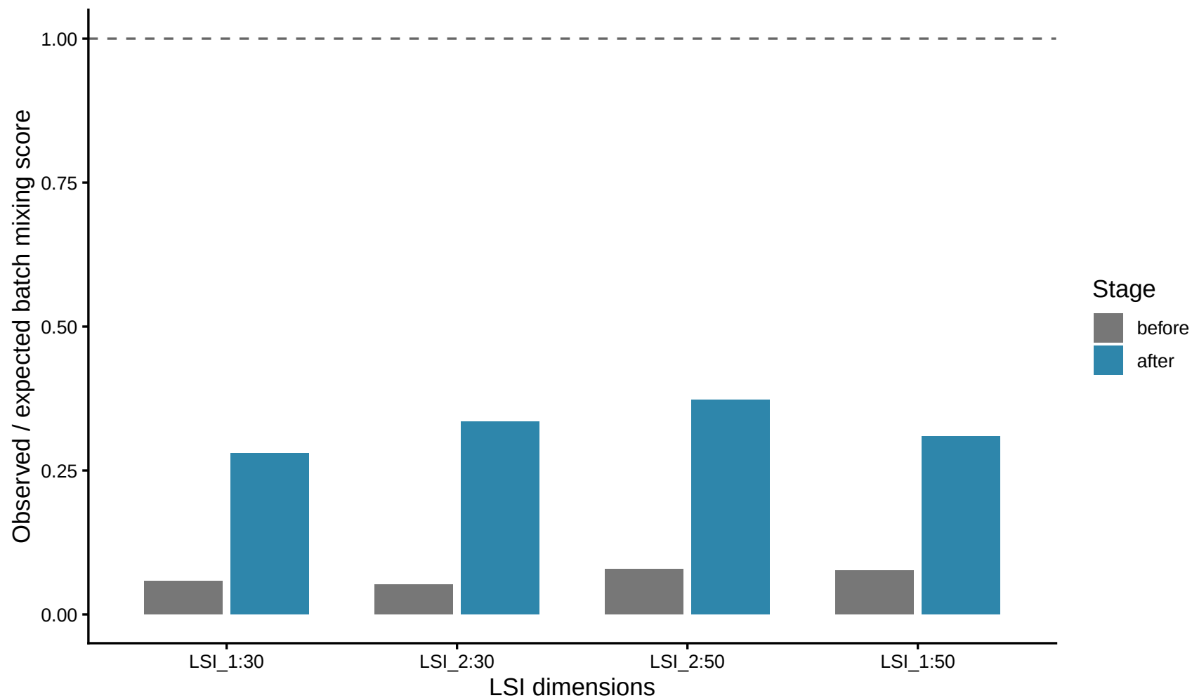
P56 LSI dimension sensitivity for paper-style batch mixing score
