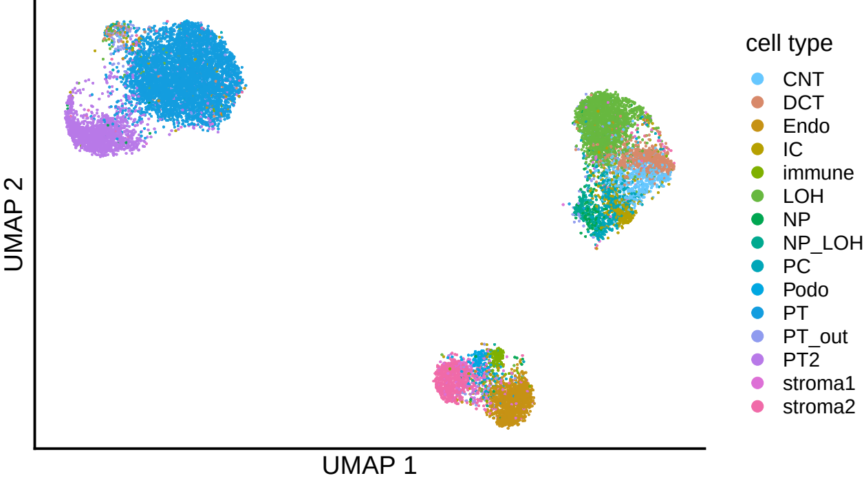
P56 after PACS batch-peak filtering by cell type
