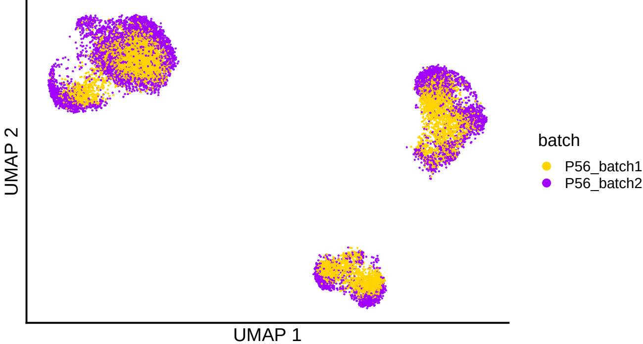
P56 after PACS batch-peak filtering by batch
