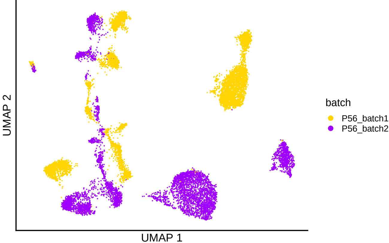
P56 before PACS filtering by batch
