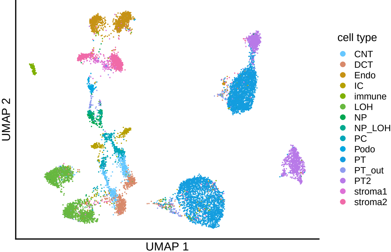
P56 before PACS filtering by cell type
