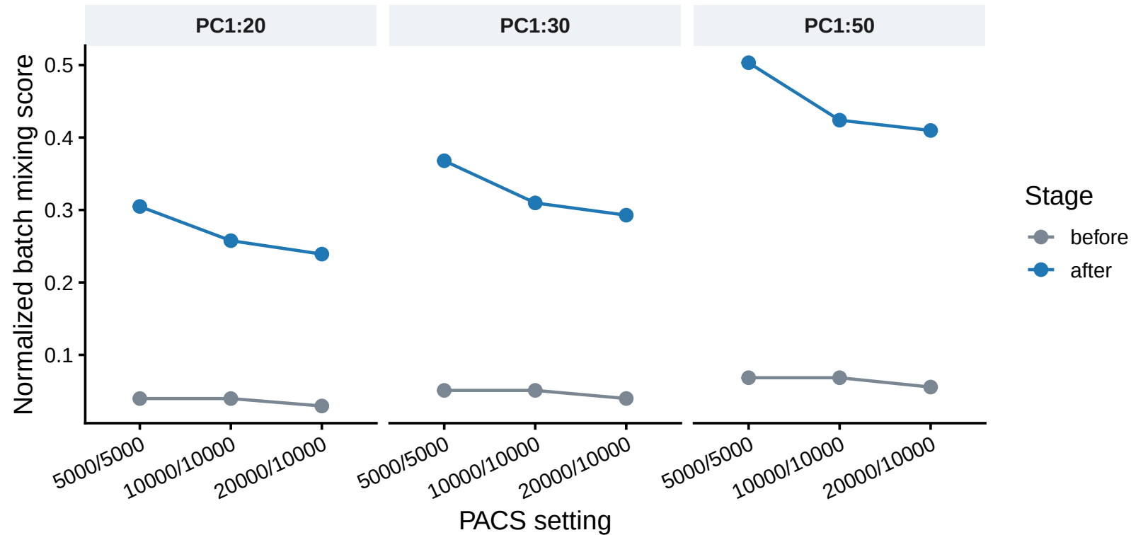
P56 PCA-logNorm paper-style batch mixing parameter stability
