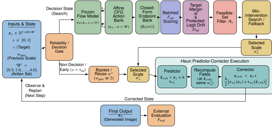
Figure 1. The CRH-CFG search-and-execute loop. At a decision state, one frozen field pair produces an affine action bank and closed-form endpoint estimates. The controller scores and filters the candidates, selects a scale, holds it through one Heun predictor-corrector pair while recomputing the field, and then replans from the corrected state. The reliability gate reuses a default or previous scale when search is bypassed. F_{eval} remains outside the control loop and measures only final outputs.
