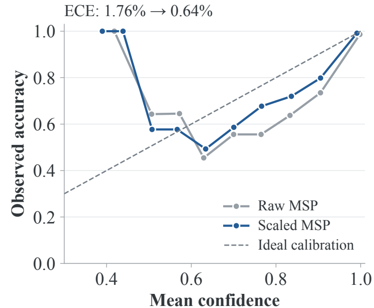
(a) Reliability before and after scaling
