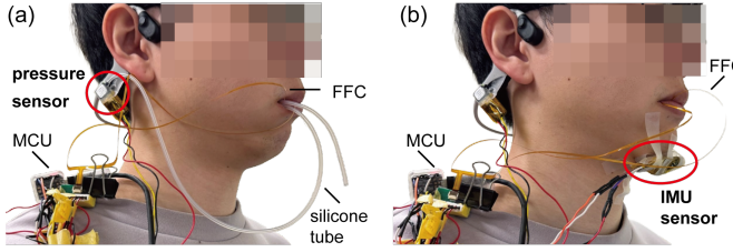
Fig. 5. Sensor configurations for mastication-phase detection. (a) Pressure-based detection in the silicone tube condition. (b) IMU-based detection in the gummy candy condition, in which participants chewed the gummy candy with the molars on the stimulated side. In both setups, sensor signals were processed by the MCU to trigger phase-dependent stimulation.
