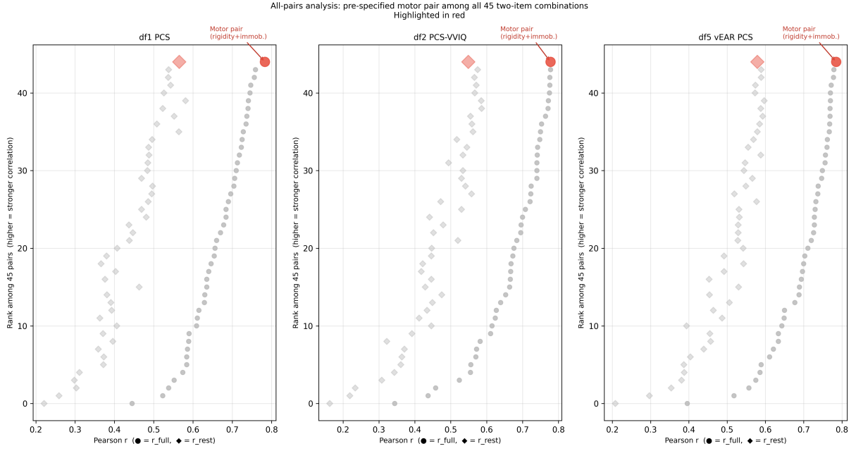
Figure 5: All 45 two-item combinations ranked by r_{full} (circles) and r_{rest} (diamonds) across three PCS datasets. Motor pair in red.
