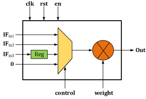
Fig. 4. Processing Element
