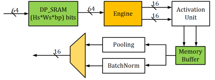
Fig. 6. Proposed Processing Core
