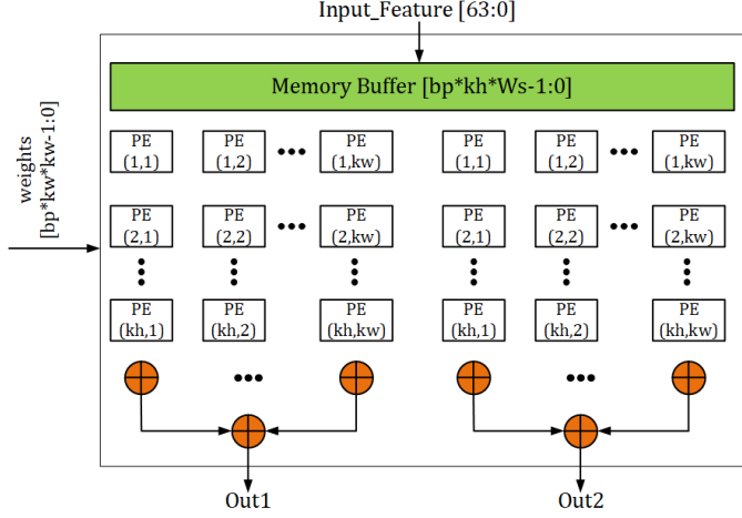
Fig. 5. Proposed Processing Engine
