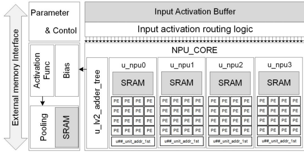
Fig. 2. Hardware configuration of Neural Engine for VGG-16 [6]
