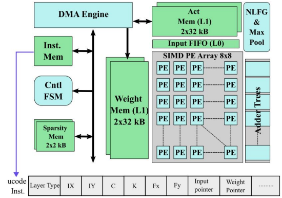
Fig. 3. Top Level architecture for DLA based on GEMM [8]
