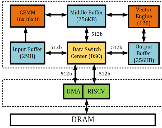
Fig. 1. Top Level architecture for DLA based on GEMM [5]
