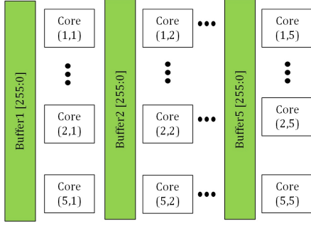
Fig. 7. Proposed Accelerator (The Mega Core)
