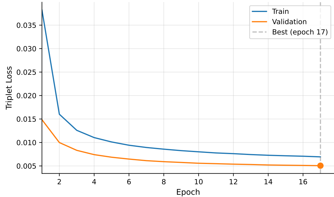
Phase 3: Hard Negative Fine-tuning
