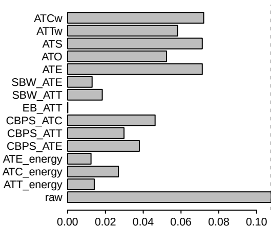
Mean Abs. Std. Mean Diffs.
