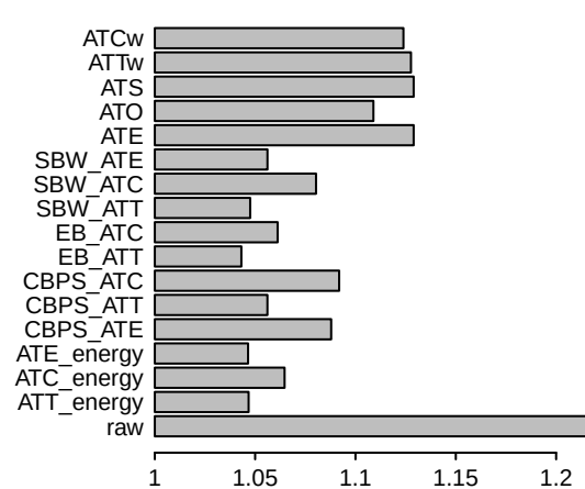
Geom. Mean Var. Ratio
