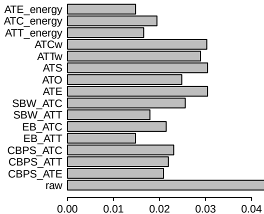
Mean KS Test Statistic
