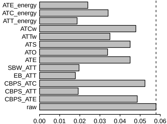
Mean KS Test Statistic
