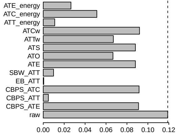
Mean Abs. Std. Mean Diffs.
