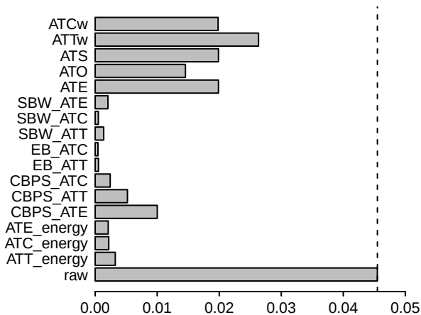
Mean Abs. Std. Mean Diffs.
