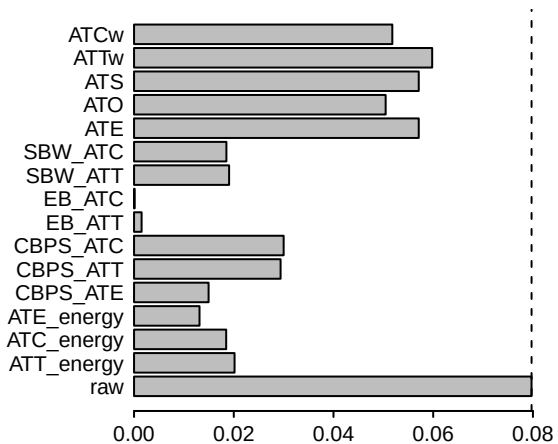
Mean Abs. Std. Mean Diffs.
