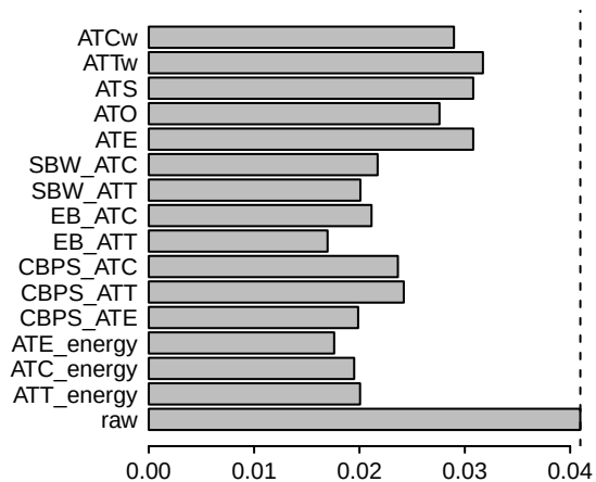
Mean KS Test Statistic
