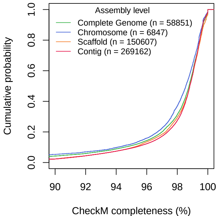
Fig1B CDF of CheckM completeness
