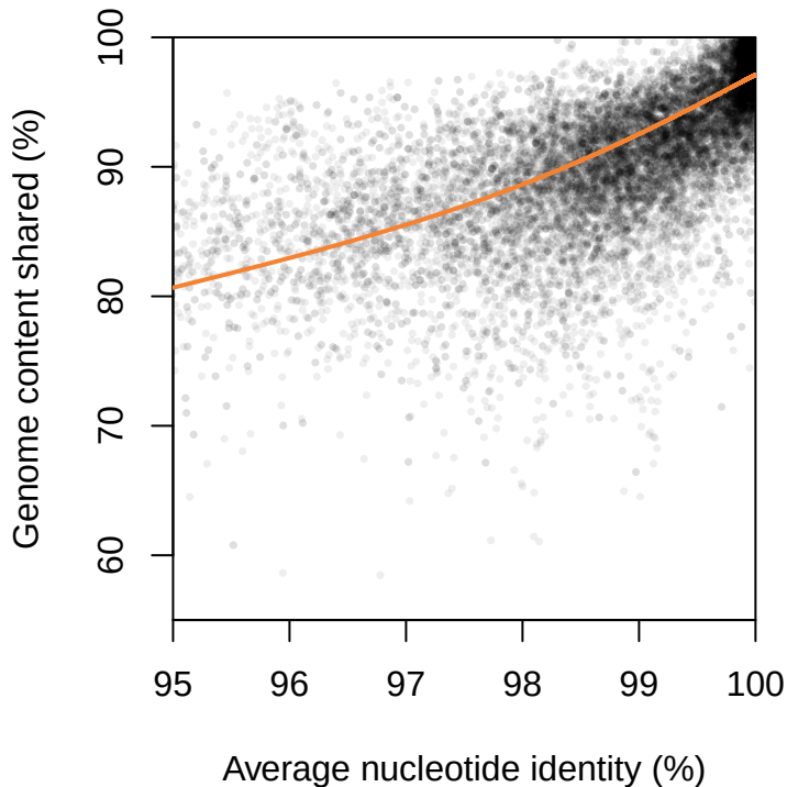
Fig2B. ANI vs. AF (fastANI fragLen3000) x=100 intercept: 97.1169
