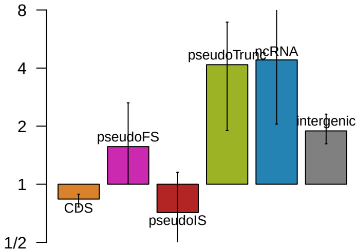
Fig5B. Feature enrichment in Ronly mapped region
