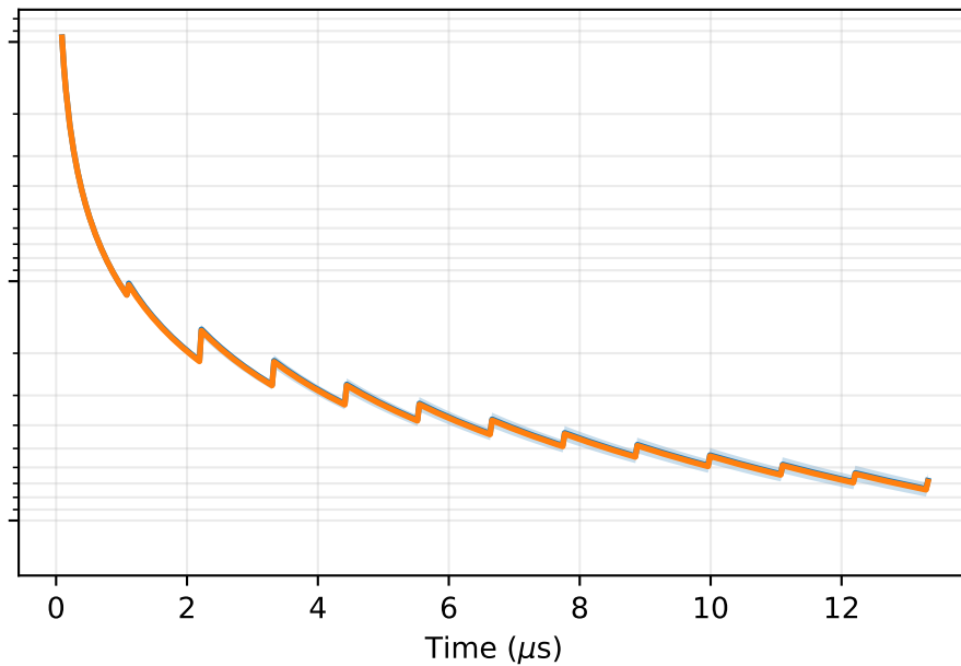
4-qubit (sequential)
