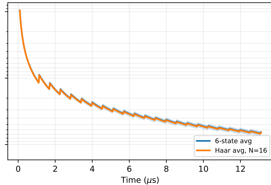
5-qubit (parallel)
