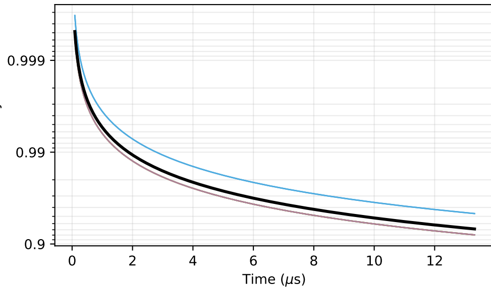
no correction
