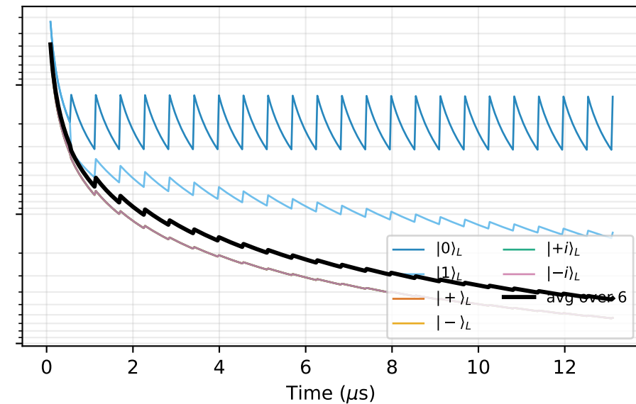
5-qubit (parallel)
