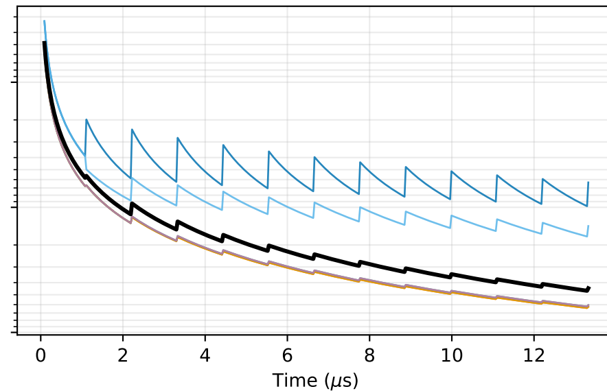
4-qubit (sequential)
