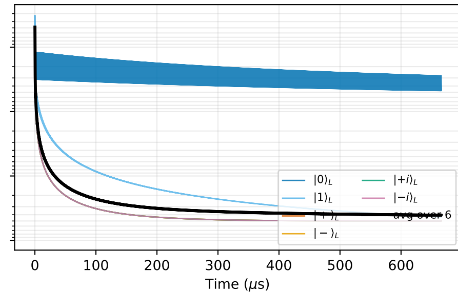
5-qubit (parallel)
