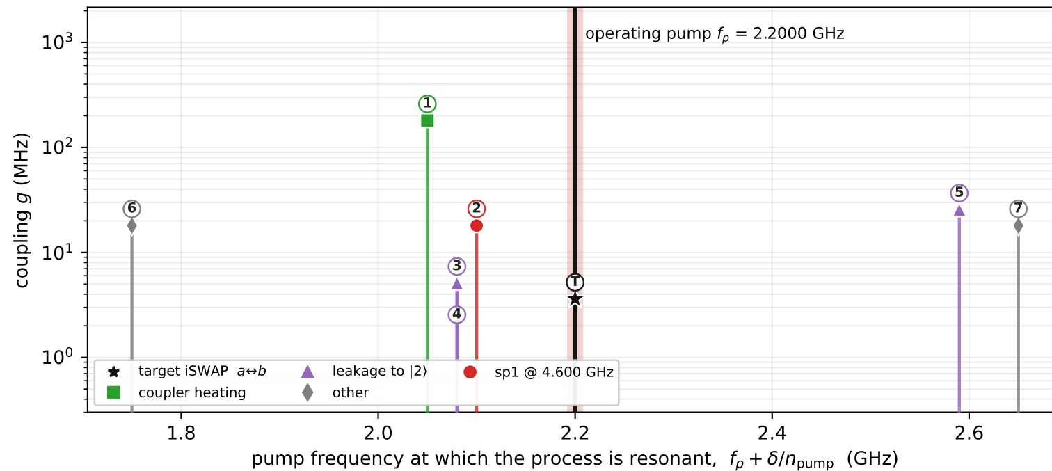
Interaction landscape — evan_device.json t_g=138.9 ns, peak |\eta|=1.00
