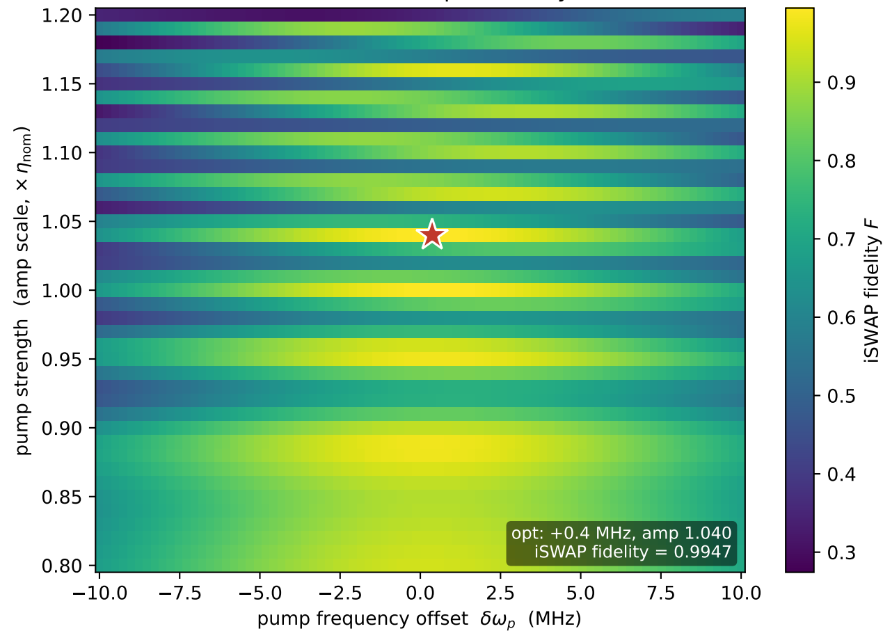
iSWAP calibration landscape (fidelity, reduced)
