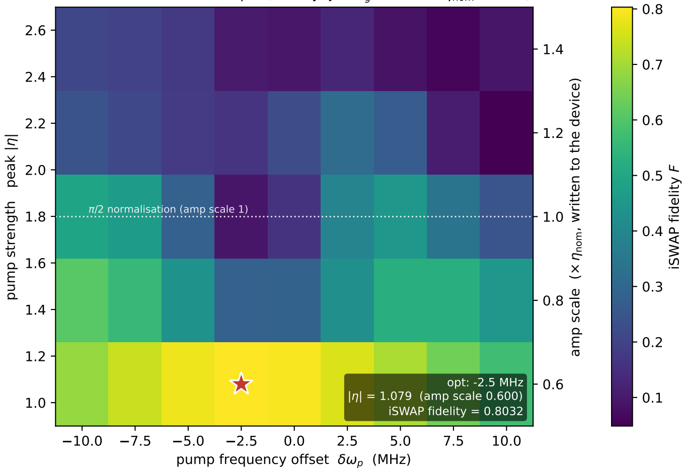
iSWAP calibration landscape (fidelity, jax, t_g=77.2 ns, \eta_{\text{nom}}=1.799 )
