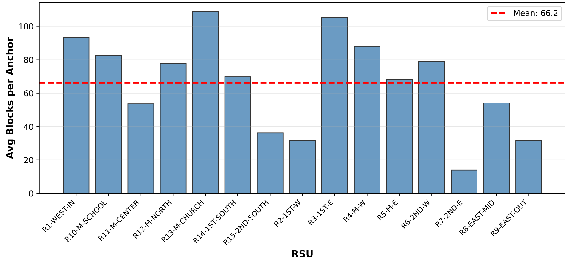
RSU Anchoring Performance (600s Test)
