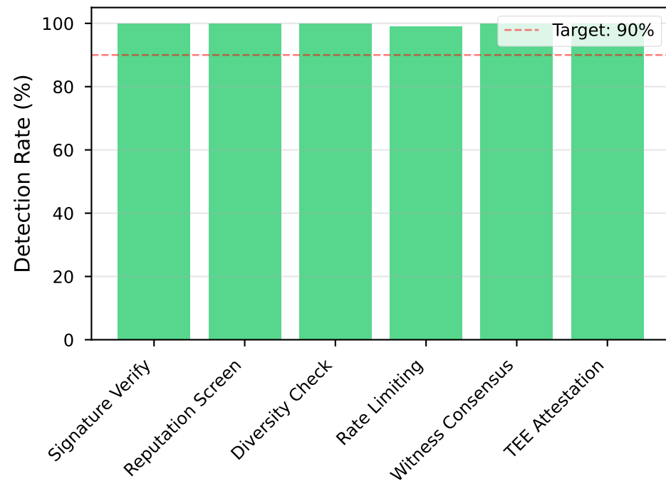
(a) True Positive Rate (Detection)
