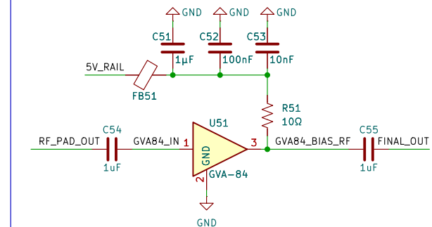
RF Gain Stage (50-series PNs)
