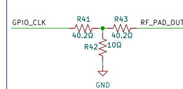
20 dB 50 Ω Attenuator Pad (40-series PNs)
