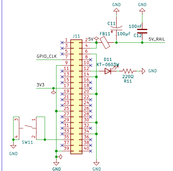
PI Control Circuit (10-series PNs)
