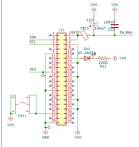
Pi Control Circuit (10-series PNs)
