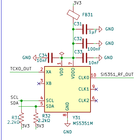
SI5351 Clock Source (30-series PNs)
