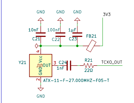
XTAL Circuit (20-series PNs)
