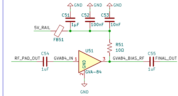
RF Gain Stage (50-series PNs)
