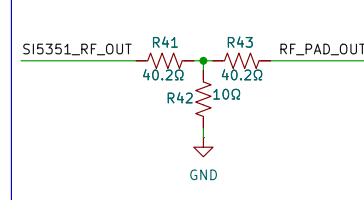
20 dB 50 Ω Attenuator Pad (40-series PNs)
