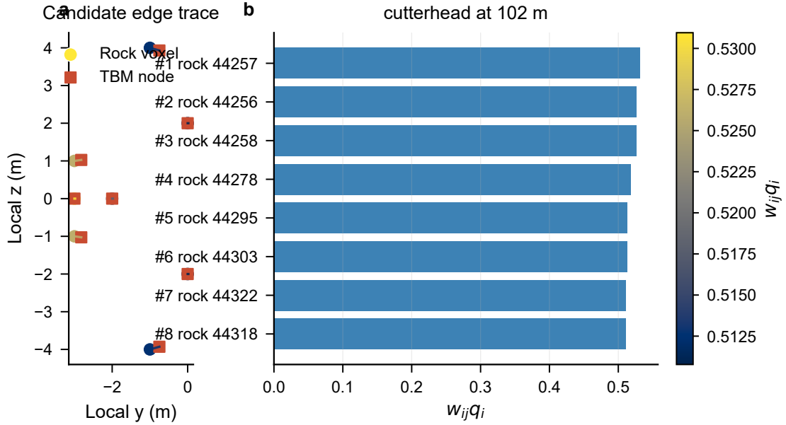
Figure 8: Traceability example for a primary diagnostic pair. Candidate rock-machine edges are ranked by w_{ij}^m(t)q_i , showing how the component-chainage descriptor can be traced back to individual rock voxels and TBM surface nodes.
