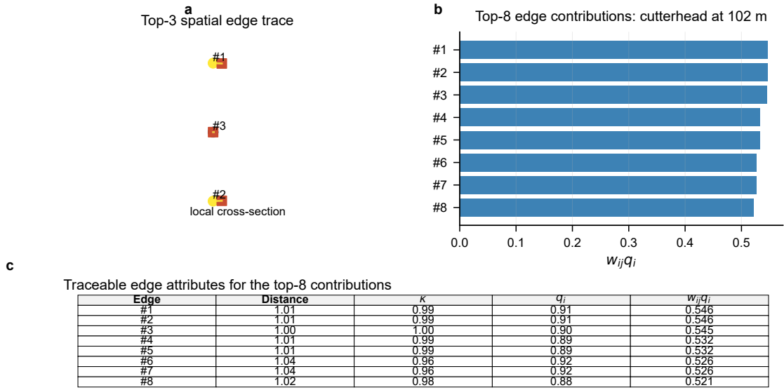
Figure 7: Traceability example for a fixed diagnostic pair. Candidate rock-machine edges are ranked by w_{ij}^{rm}(t)q_i , showing how the component-chainage descriptor can be traced back to individual rock voxels and TBM surface nodes.
