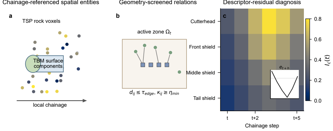
Figure 1: Workflow of the chainage-referenced rock–TBM spatial interaction graph. The figure summarises how spatial entities are aligned, how geometry-screened candidate relations are constructed, and how component–chainage descriptors are evaluated against persistence residuals.
