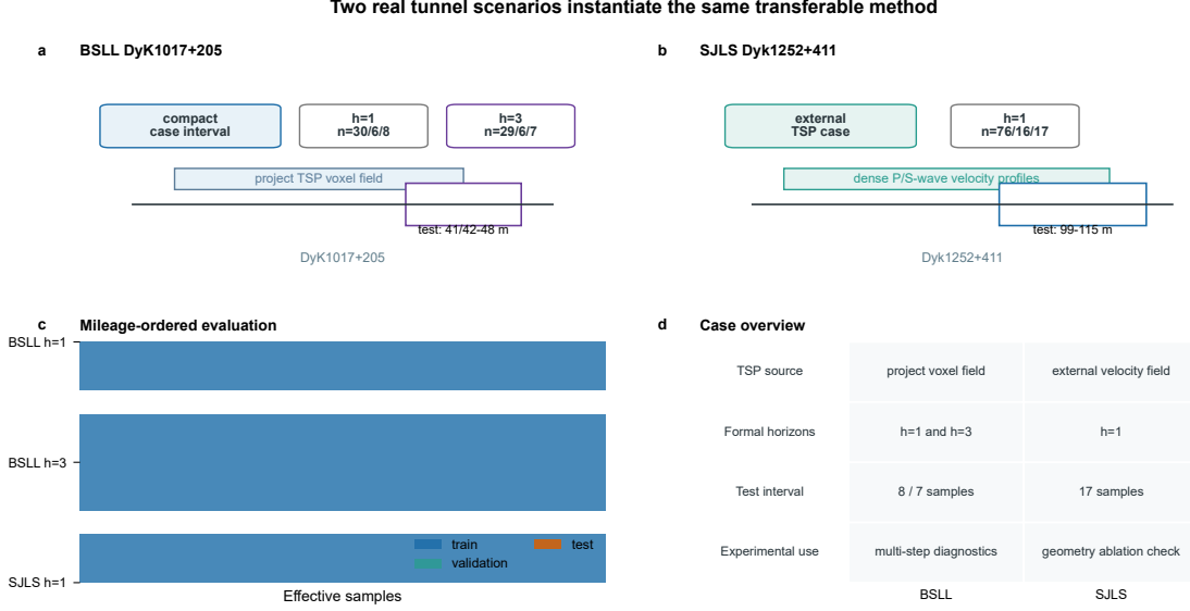
Figure 3: Real tunnel scenarios used to instantiate the common descriptor framework. BSLl DyK1017+205 provides compact h=1 and h=3 cases, while SJLS Dyk1252+411 provides the strongest external TSP descriptor evidence.
