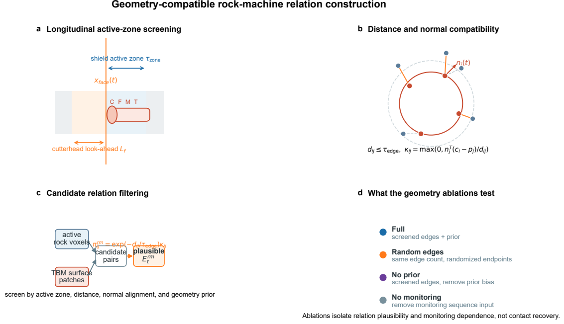
Figure 2: Geometry-constrained rock-machine candidate relation construction. Candidate relations are controlled by active-zone membership, distance decay, surface-normal compatibility, and excavation state. The construction defines spatially plausible relations; it does not recover measured contact.
