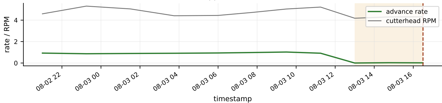
D. Event window: advance approaches zero while cutterhead rotates
