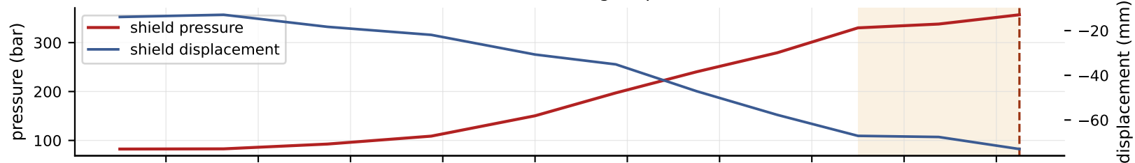
C. TBM monitoring response
