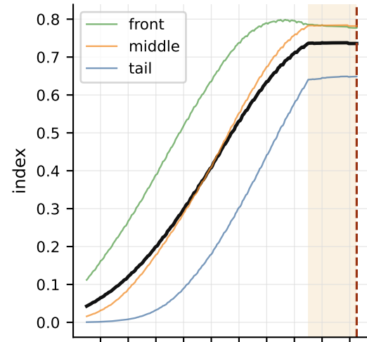
C. Component-level shield index
