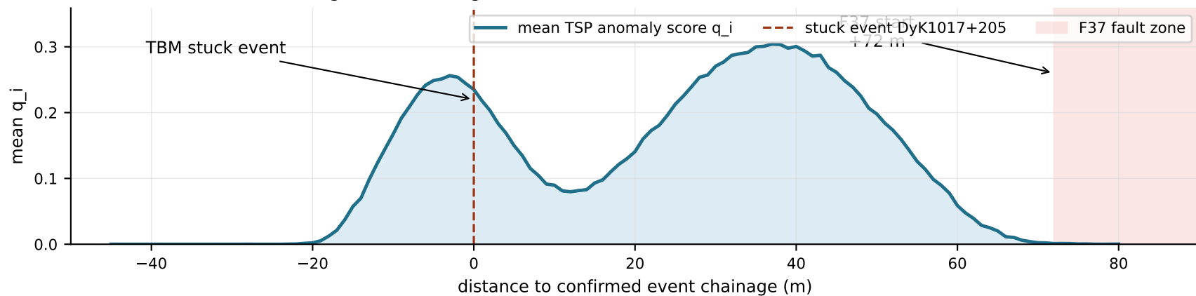
A. Longitudinal setting: event location, TSP anomalies and F37 fault influence
