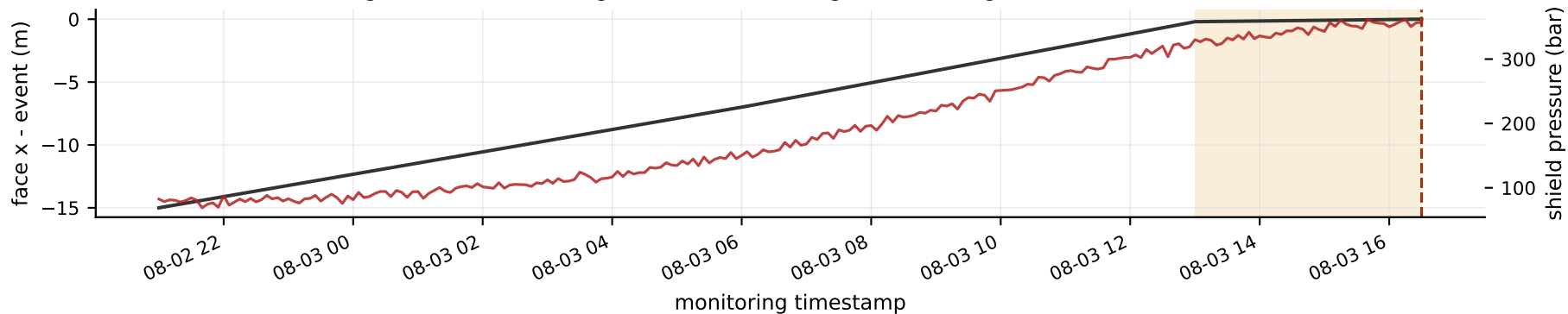
C. Alignment: TSP chainage, TBM face chainage, monitoring time and event window
