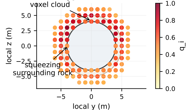
B. Cross-section: shield, surrounding rock and low-velocity voxels near the event
