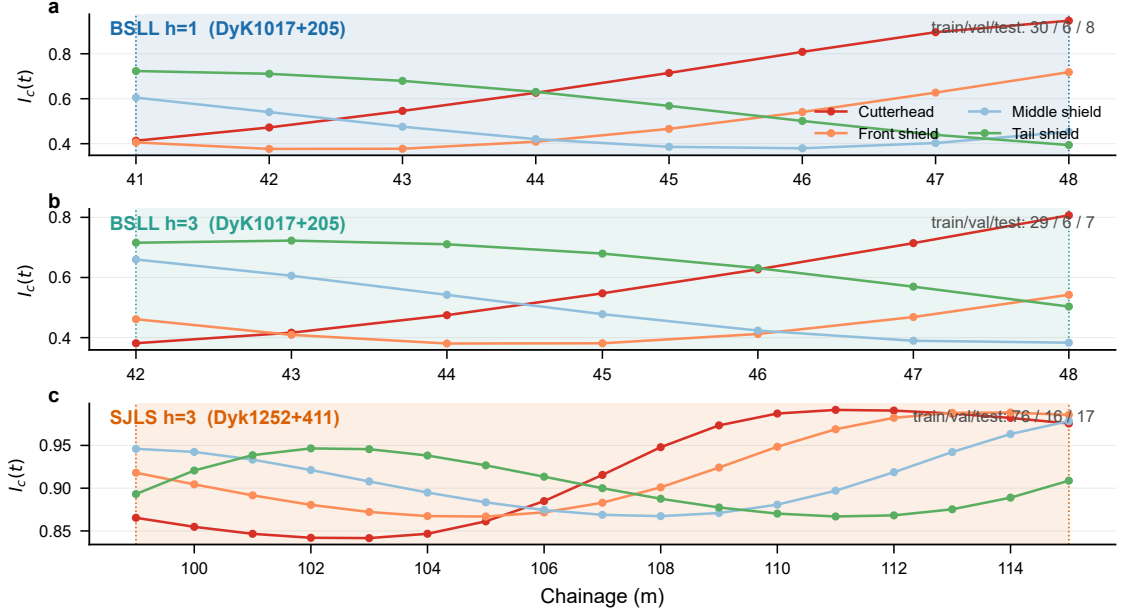
Figure 3: Per-component I_c(t) descriptor series for the three formal case runs on the common standardized graph support. Shaded bands mark the test chainage interval; BSL cases are compact ( n = 8, 7 ), while SJLS provides a longer test interval ( n = 17 ) with a uniformly high low-velocity anomaly level.
