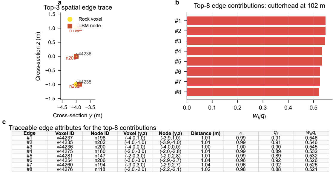
Figure 7: Traceability example for a fixed diagnostic pair. Candidate rock-machine edges are ranked by w_{ij}^{rm}(t)q_i , showing how the component-chainage descriptor can be traced back to individual rock voxels (labelled by voxel ID and cross-section coordinates) and TBM surface nodes (labelled by node ID and coordinates). The table reports the top-8 contributing edges with their voxel ID, node ID, voxel and node (y, z) positions, edge distance, normal compatibility \kappa , anomaly score q_i , and weighted contribution.
