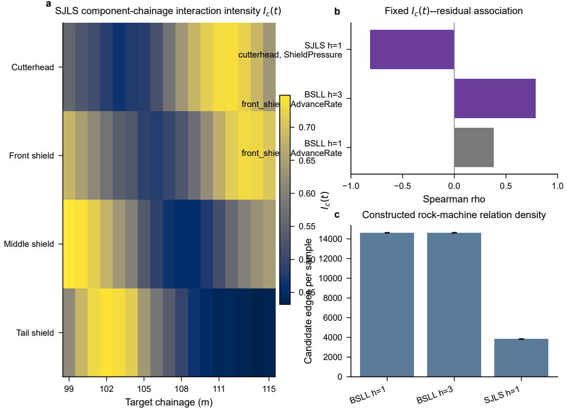
Figure 4: Component-chainage spatial interaction descriptor evidence. Panel (a) shows SJLS I_c(t) values aggregated from geometry-weighted TSP anomaly scores over candidate rock-machine relations. Panel (b) reports the fixed I_c(t) –persistence-residual association used in the threshold sensitivity analysis. Panel (c) reports the mean number of constructed candidate relations per sample. The descriptors are not measured contact pressure or risk probability.
