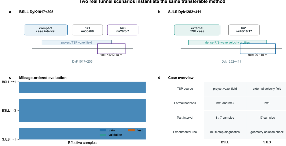
Figure 3: Real tunnel scenarios used to instantiate the common descriptor framework. BSSL DyK1017+205 provides compact h=1 and h=3 cases, while SJLS Dyk1252+411 provides the clearest external TSP descriptor evidence.
